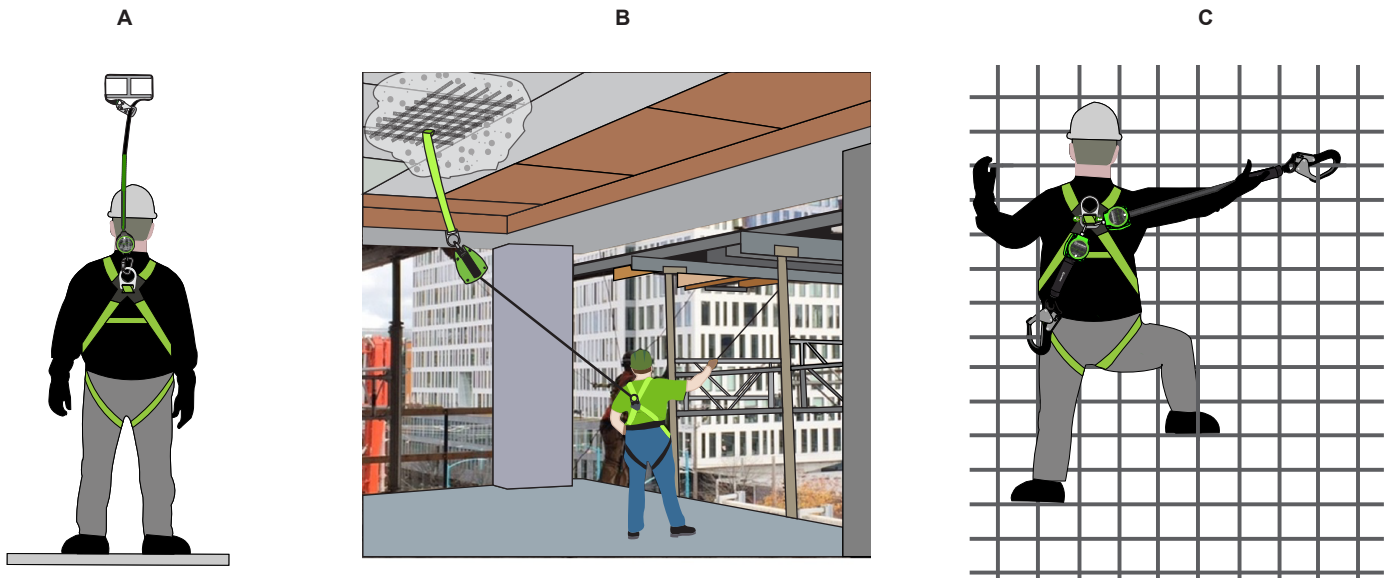
FIGURE 15 - SYSTEM CONNECTIONS
