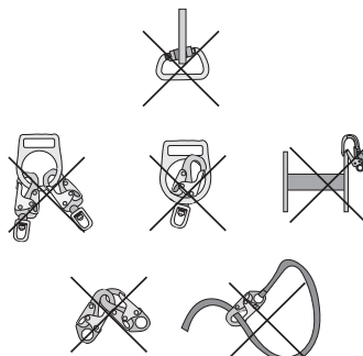
FIGURE 7 - INAPPROPRIATE CONNECTIONS
