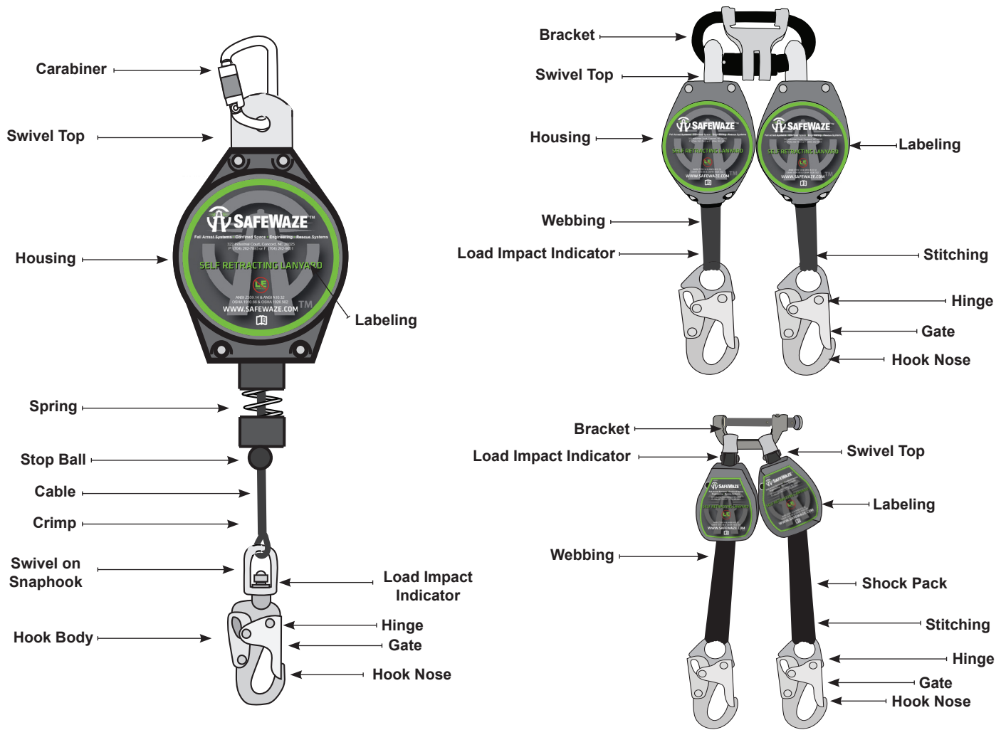
FIGURE 18 - INSPECTION DIAGRAMS
